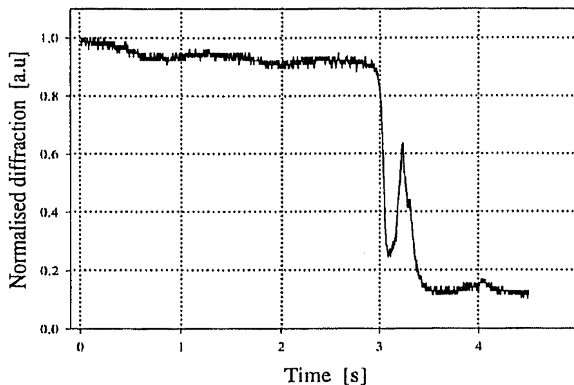
FIGURE 2 Dynamics of diffraction at phase transition at 35.2°C.
