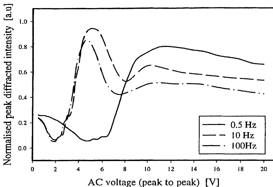
FIGURE 4 Peak diffracted intensity versus AC voltage
