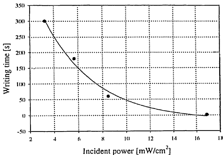
FIGURE 1 Approximate time to write a permanent grating
