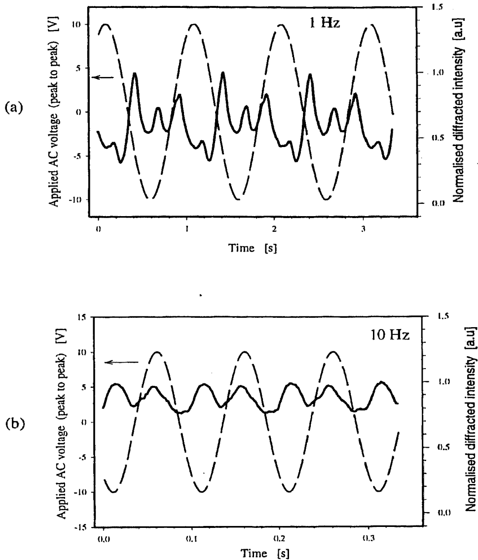
FIGURE 3 Time evolution of diffracted signal at 20 V applied AC field for different frequencies: 1 Hz (a) and 10 Hz (b)
