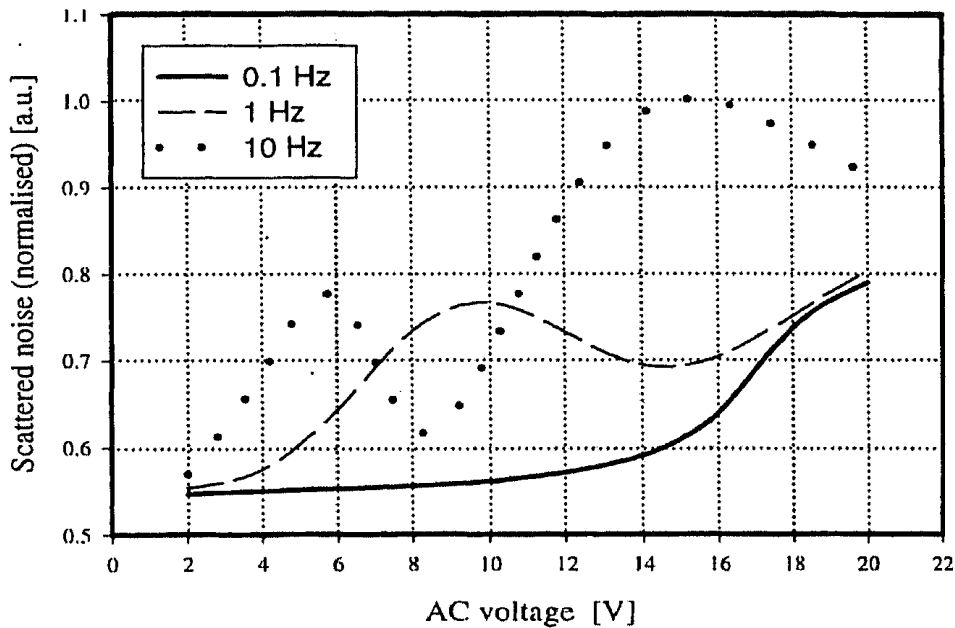
FIGURE 5 Noise (scattered light) dependence on AC field
